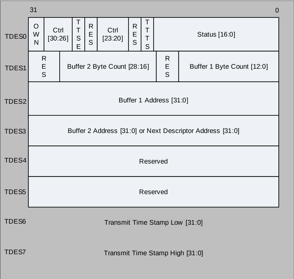
Fig 86. Transmitter descriptor fields
