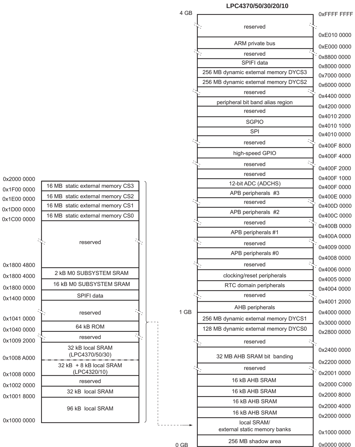
Fig 6. Flashless parts: System memory map (see Figure 7 for detailed addresses of all peripherals)
