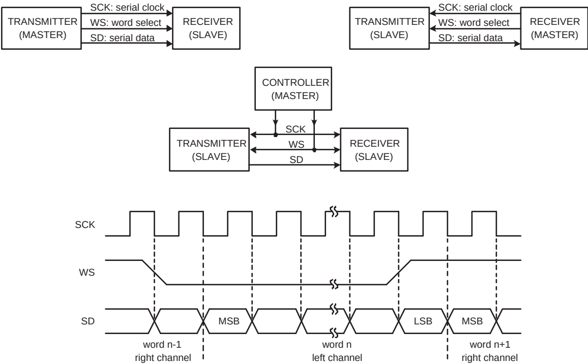
Fig 144. Simple I2S configurations and bus timing
