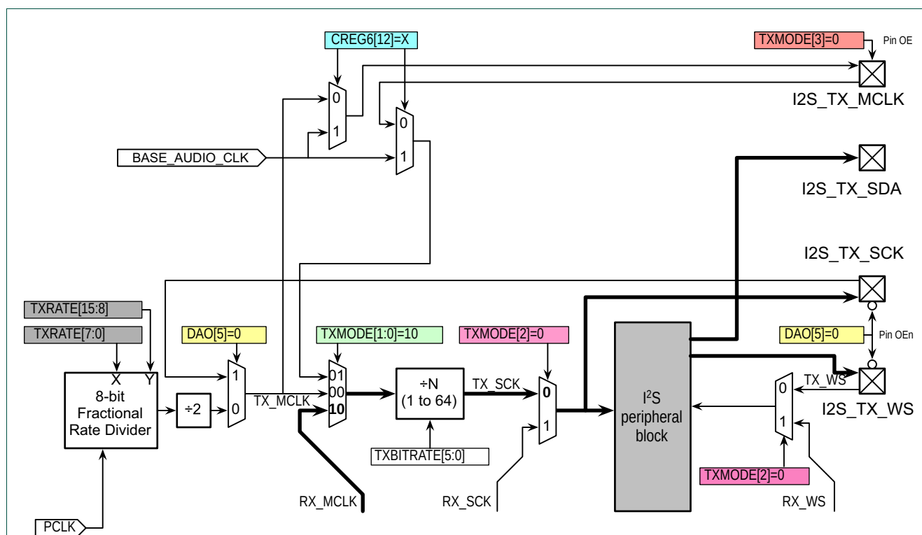
Fig 148. Transmitter master mode, sharing RX_MCLK
