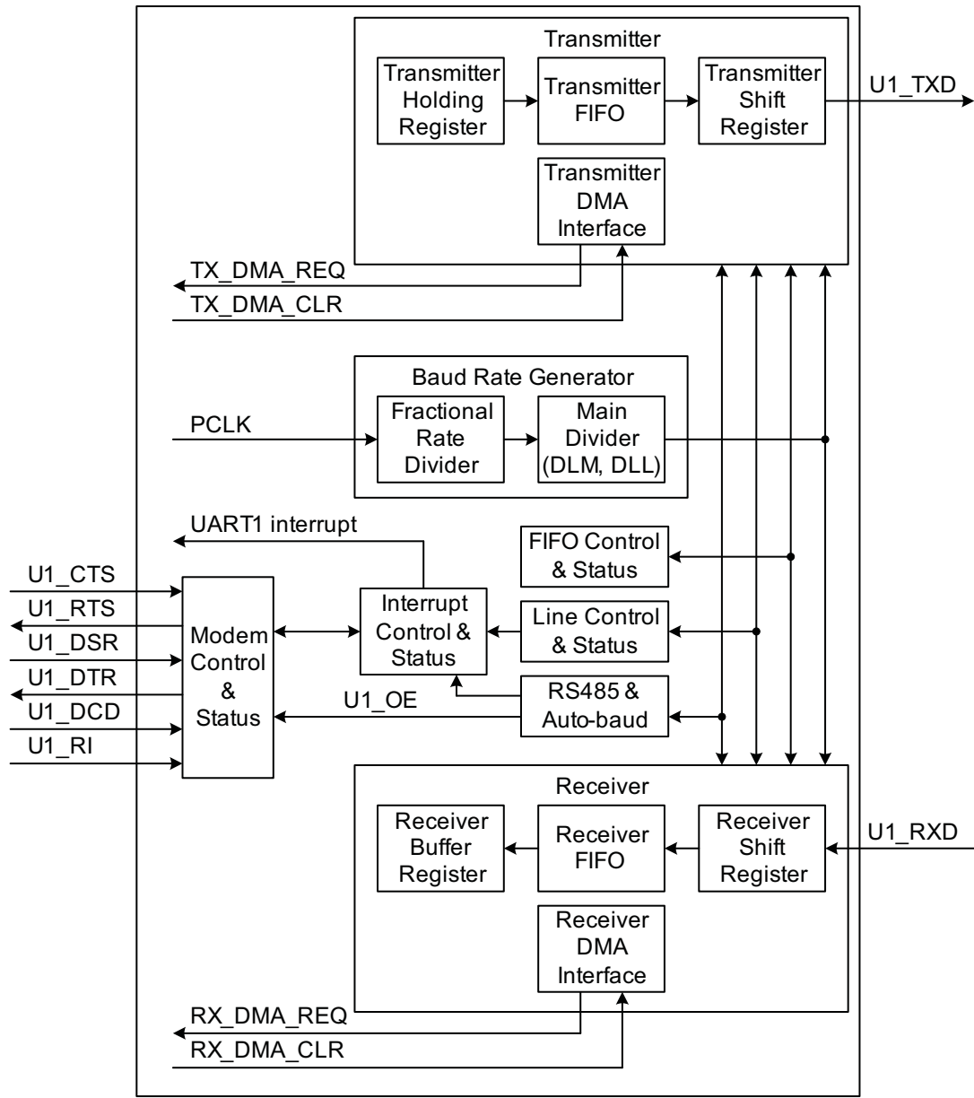
Fig 130. UART1 block diagram
