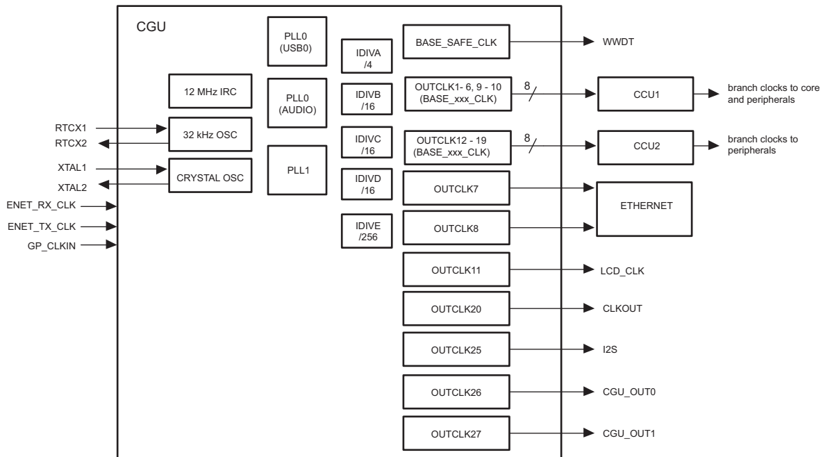
Fig 34. CGU and CCU1/2 block diagram
