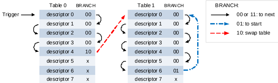
Fig 187. Using BRANCH to control the descriptor table processing order
