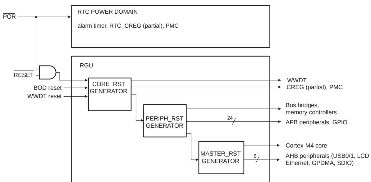
Fig 39. RGU Block diagram
