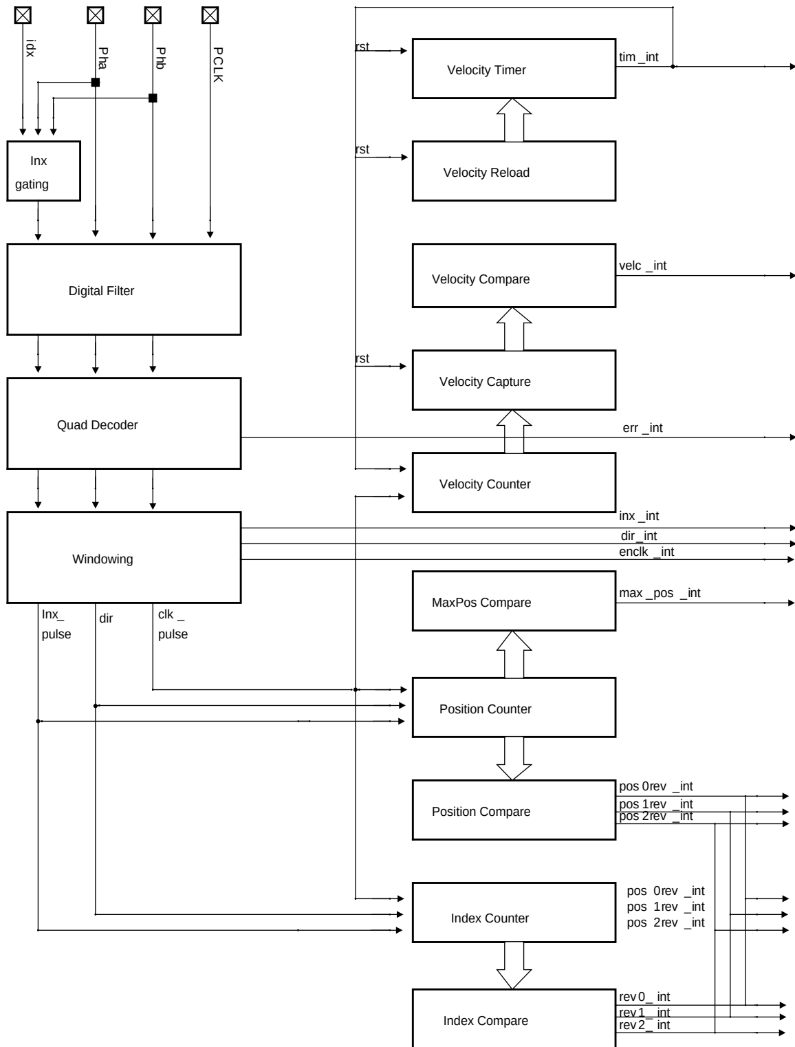
Fig 116.Encoder interface block diagram
