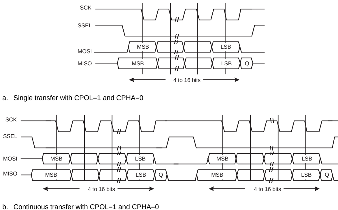
Fig 136. SPI frame format with CPOL = 1 and CPHA = 0 (a) Single and b) Continuous Transfer)
