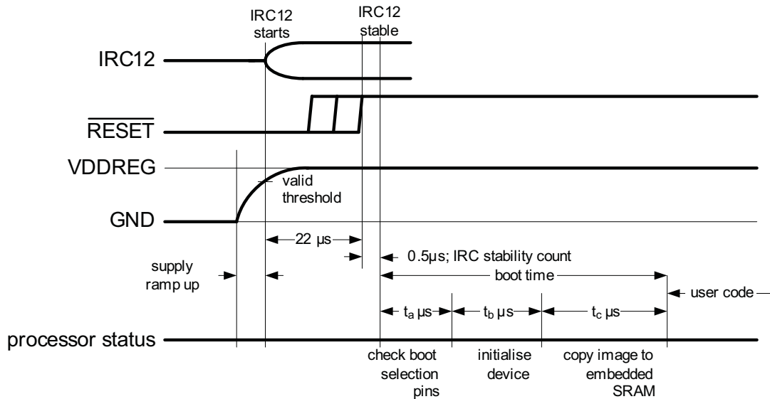
Fig 20. Boot process timing
