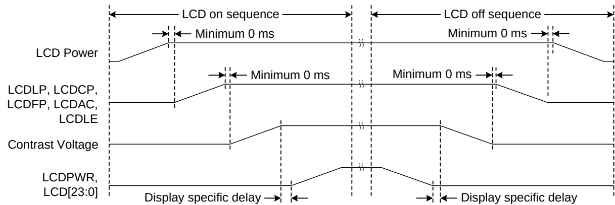
Fig 93. Power-up and power-down sequences
