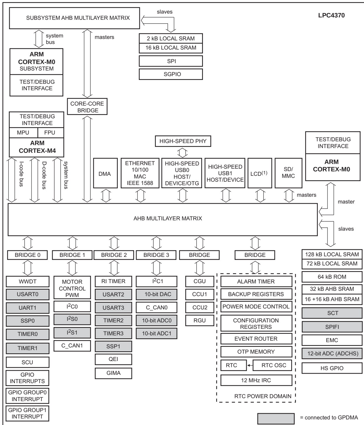
Fig 2. LPC4370 Block diagram (flashless parts, triple-core, 12-bit ADCHS)
