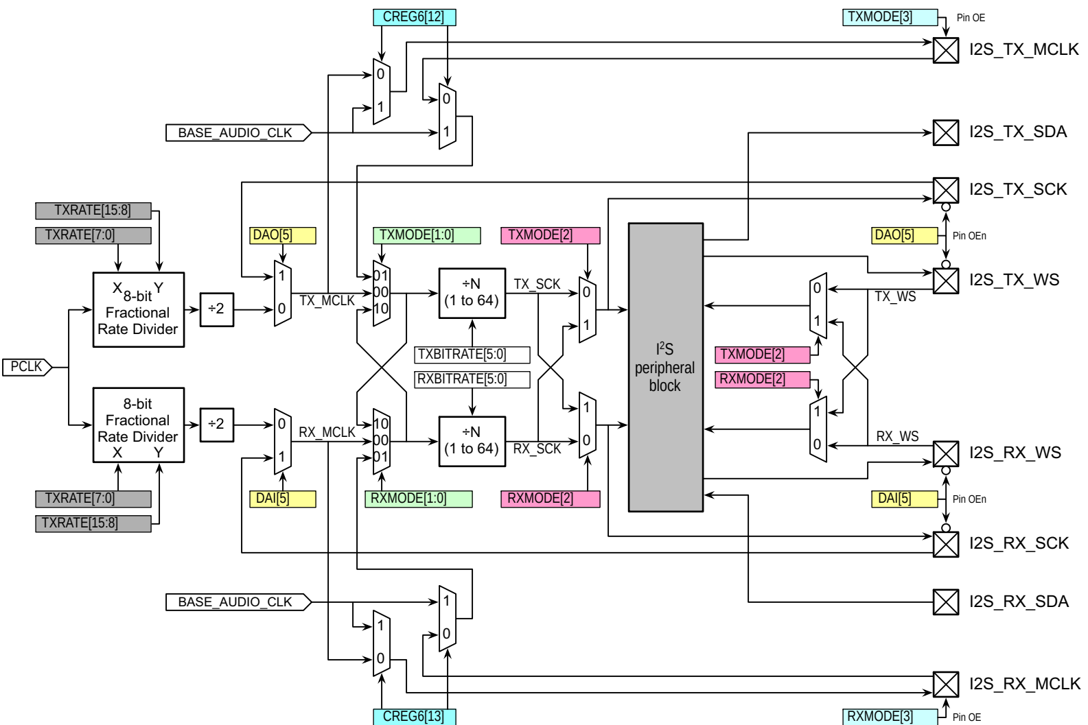
Fig 145. I2S clocking and pin connections
