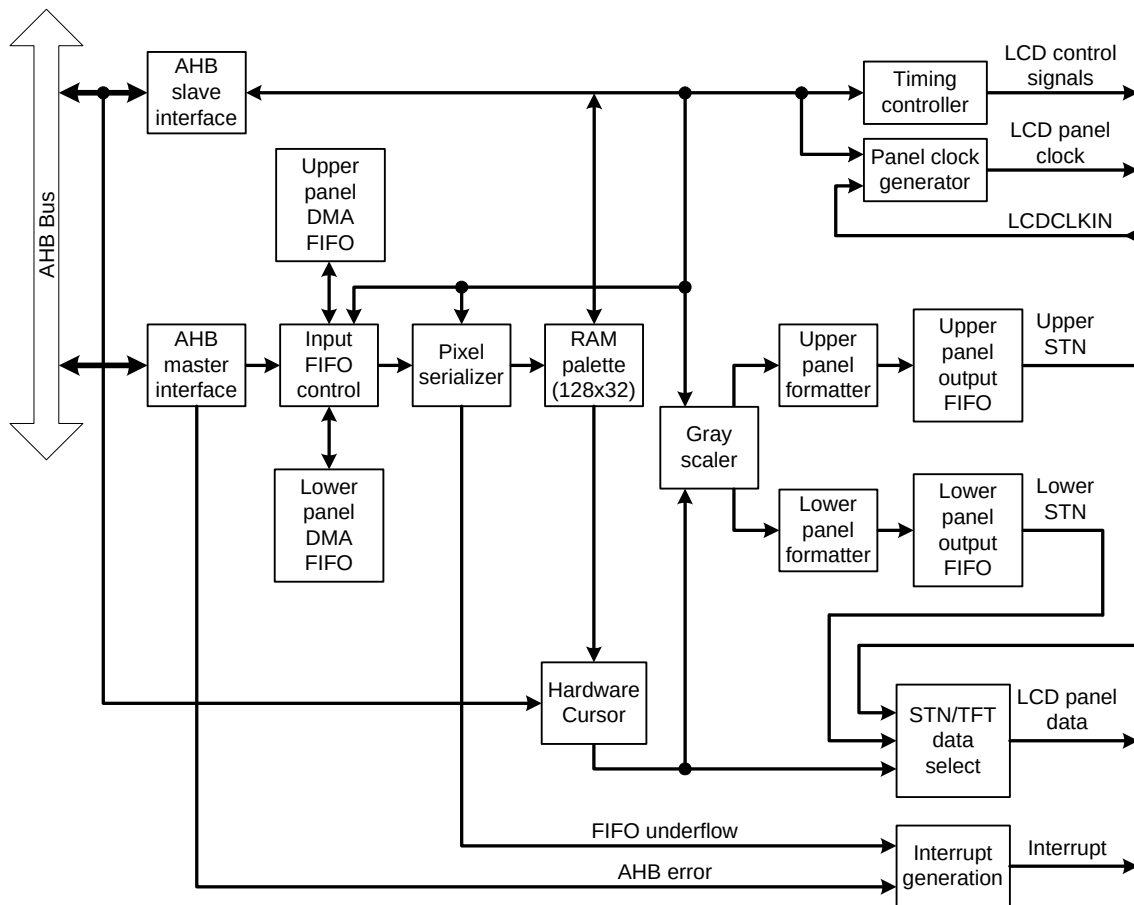
Fig 89. LCD controller block diagram
