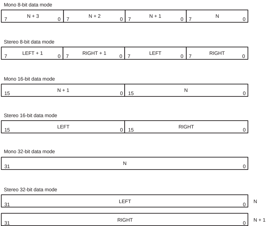
Fig 160. FIFO contents for various I2S modes
