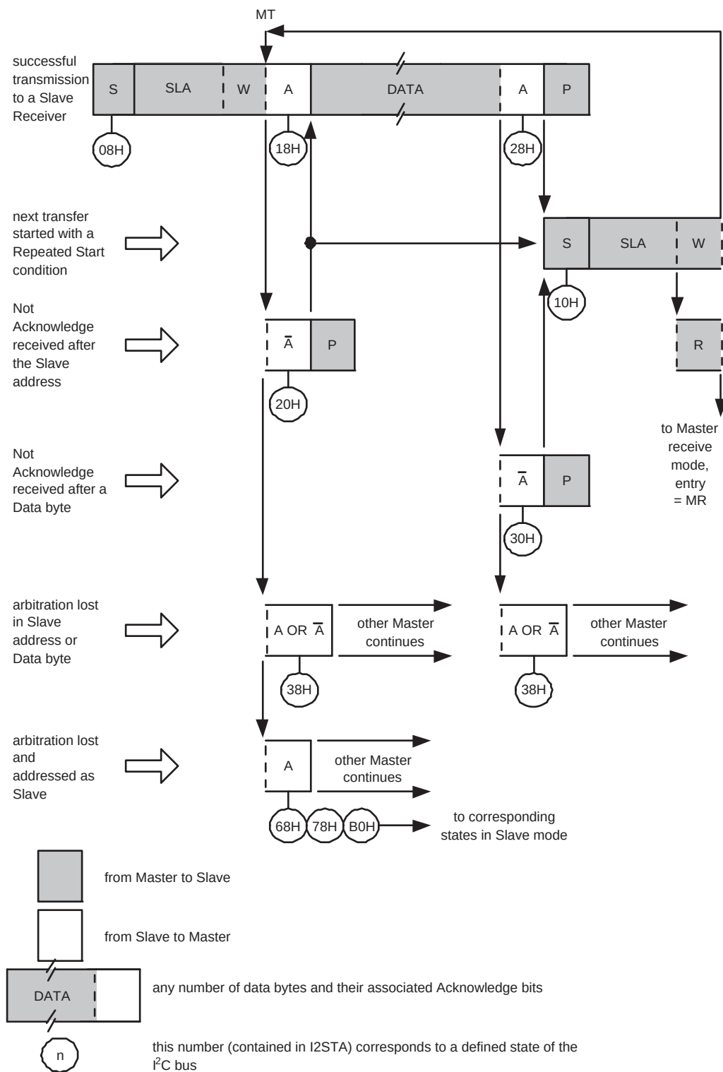
Fig 178. Format and states in the Master Transmitter mode
