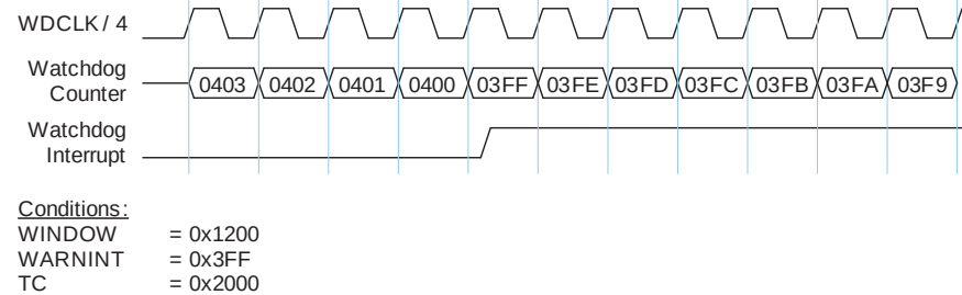
Fig 123. Watchdog Warning Interrupt
