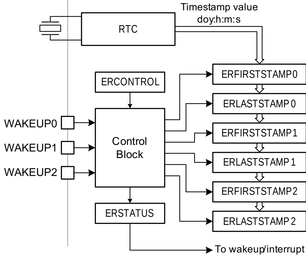
Fig 124. Event Monitor/Recorder block diagram
