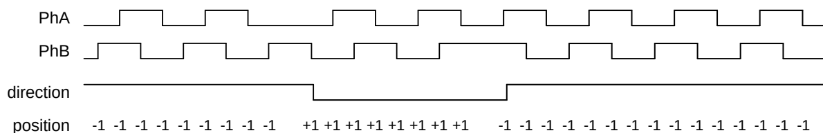
Fig 117. Quadrature Encoder Basic Operation
