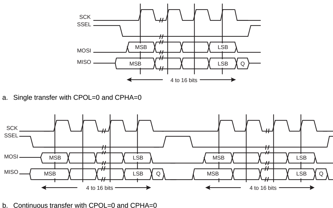
Fig 134. SPI frame format with CPOL=0 and CPHA=0 (a) Single and b) Continuous Transfer)
