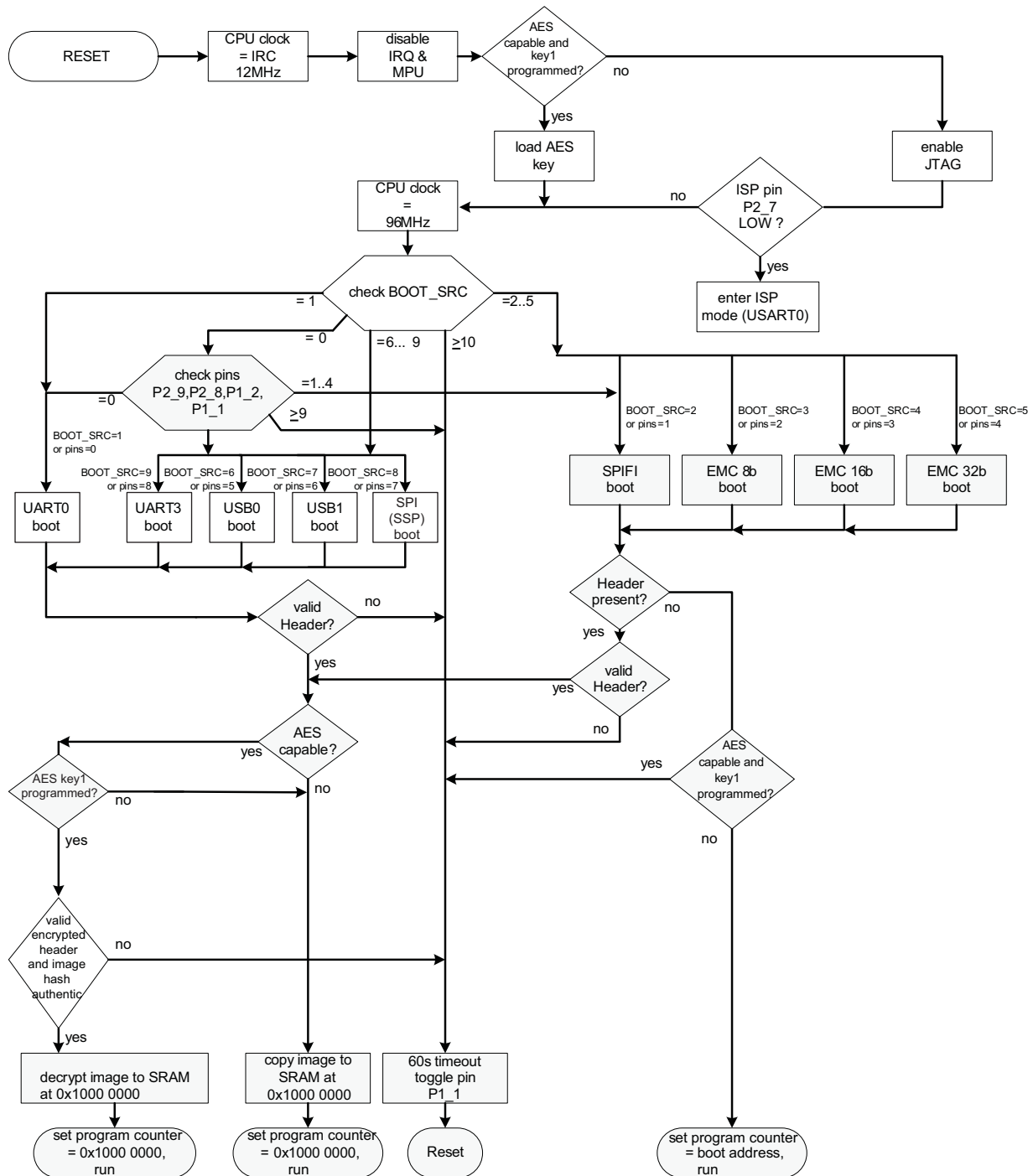
Fig 13. Boot process flowchart for LPC43xx parts with flash
