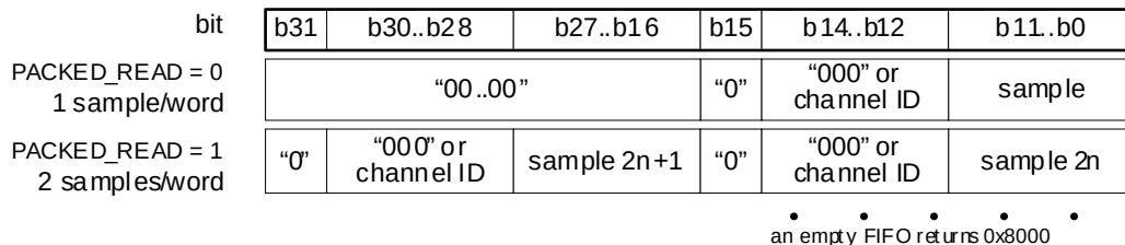
Fig 186. FIFO packed data format
