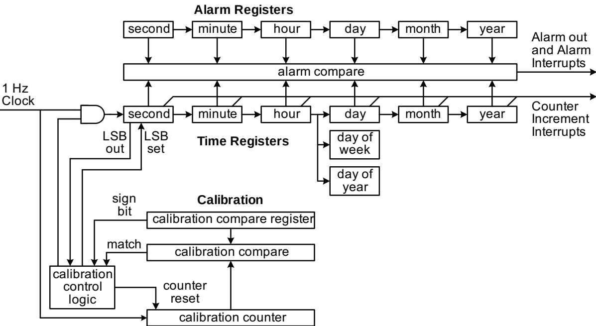
Fig 119. RTC functional block diagram
