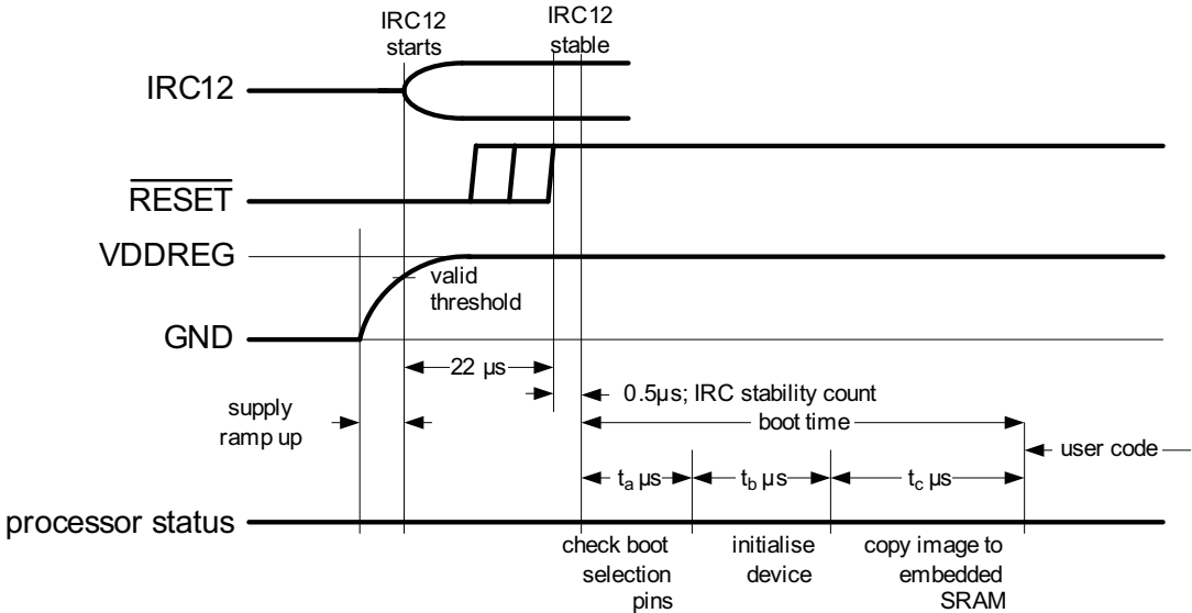
Fig 27. Boot process timing
