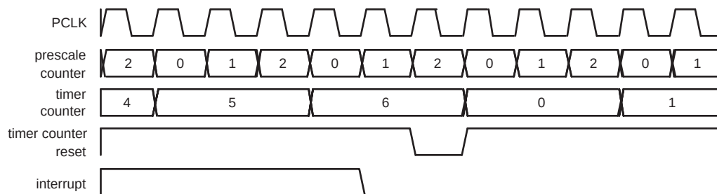
Fig 107. A timer cycle in which PR=2, MRx=6, and both interrupt and reset on match are enabled.
