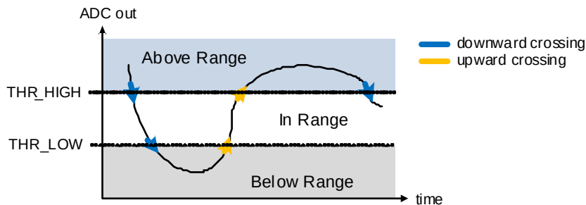
Fig 188. Threshold detection
