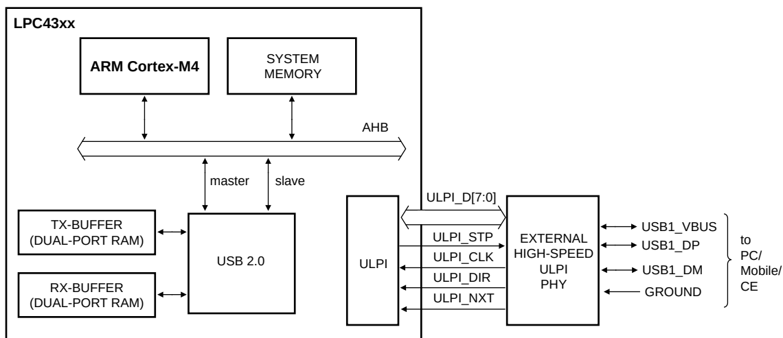
Fig 73. USB1 block diagram with ULPI
