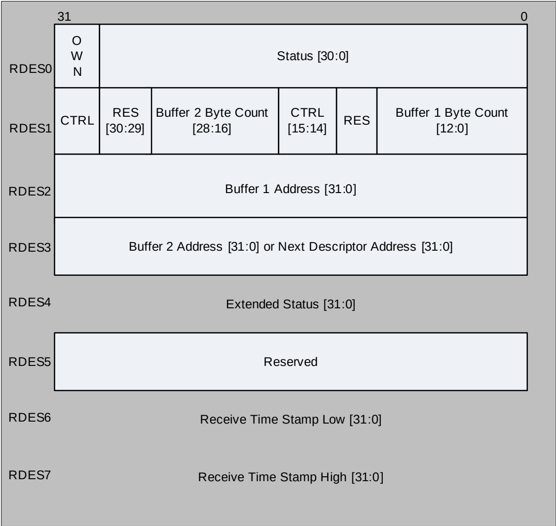
Fig 88. Receive descriptor fields (alternate configuration)
