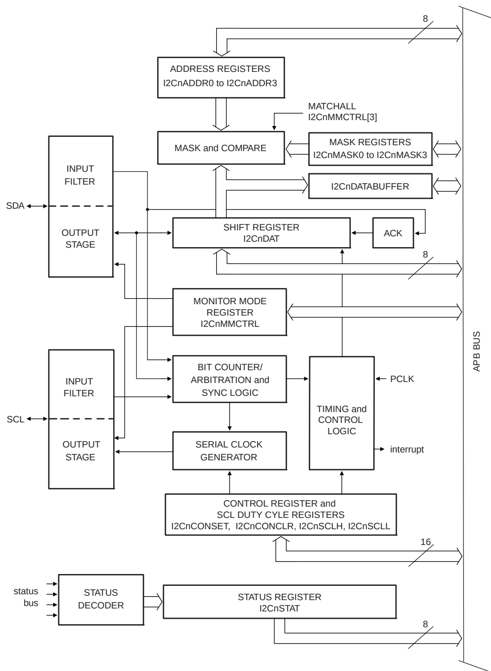
Fig 175. I 2 C serial interface block diagram
