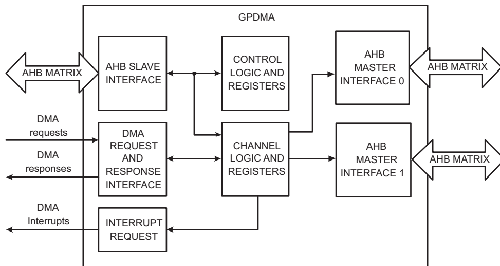
Fig 52. DMA controller block diagram
