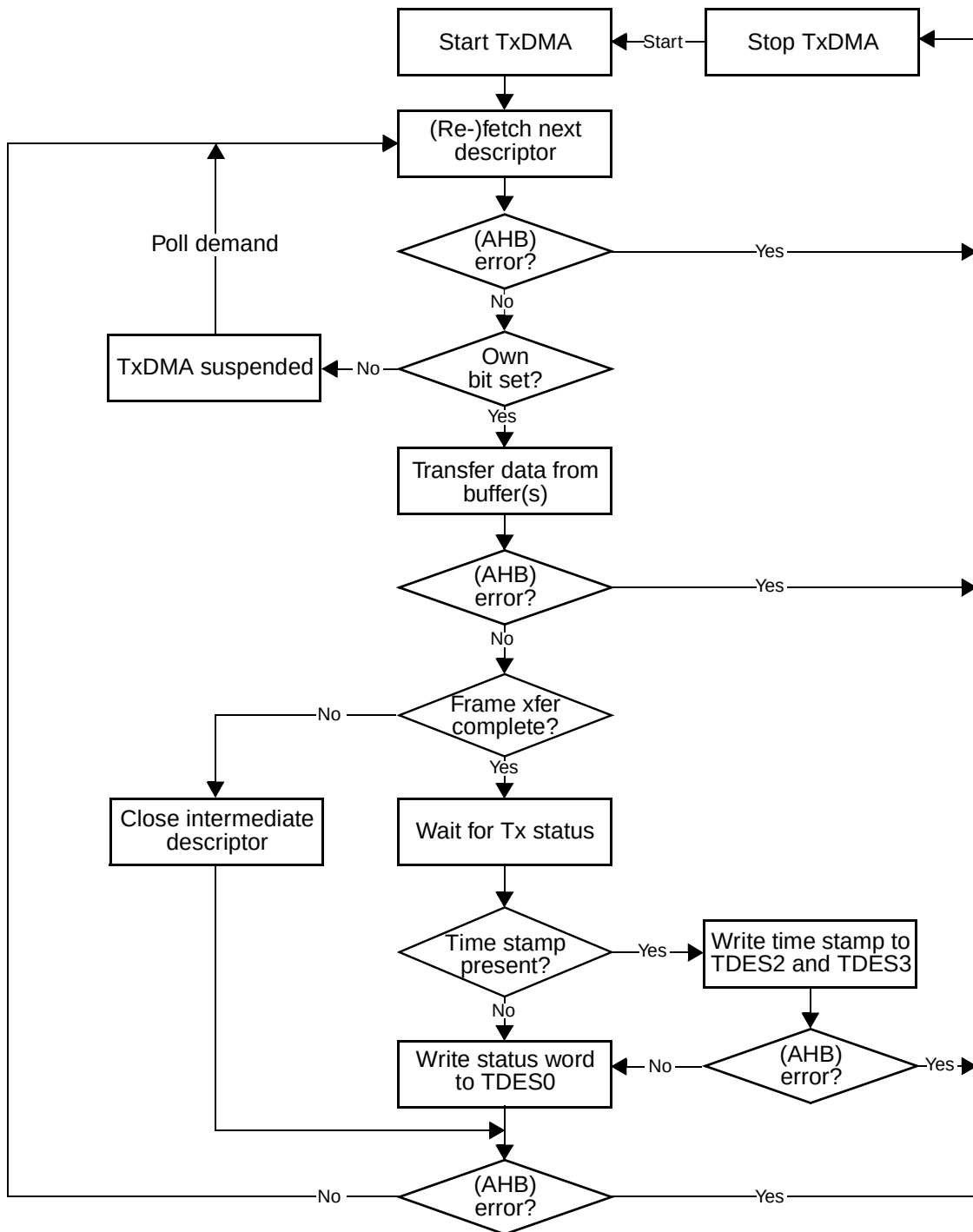
Fig 83. TxDMA operation in default mode
