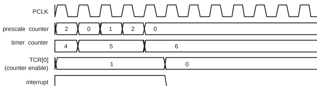
Fig 108. A timer Cycle in Which PR=2, MRx=6, and both interrupt and stop on match are enabled
