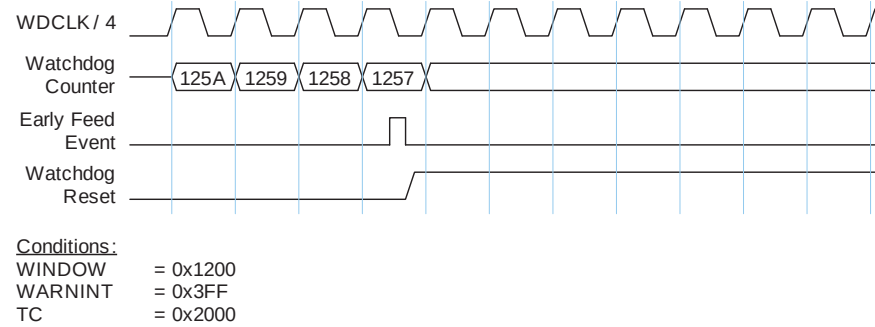
Fig 121. Early Watchdog Feed with Windowed Mode Enabled
