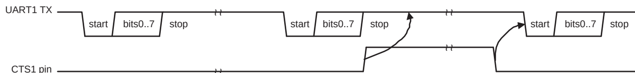
Fig 132. Auto-CTS Functional Timing
