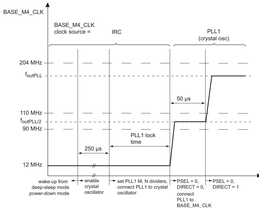
Fig 33. BASE_M4_CLK ramp-up procedure
