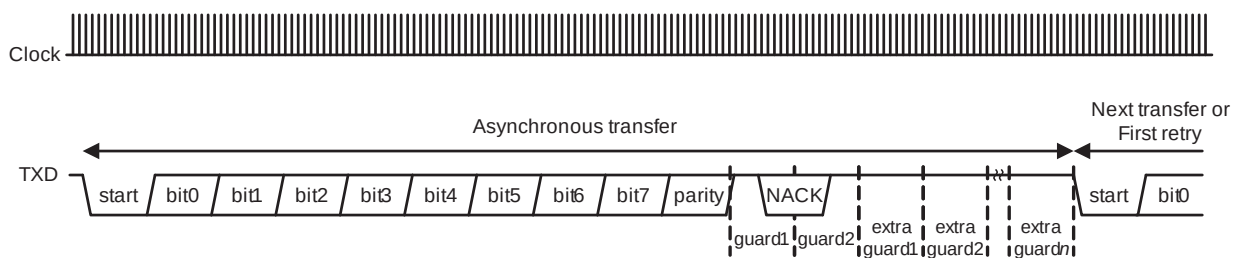
Fig 129. Smart card T = 0 waveform
